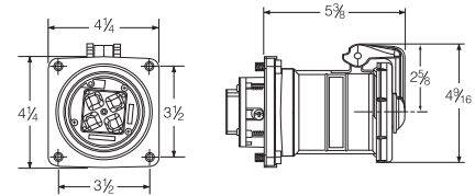
Plug
