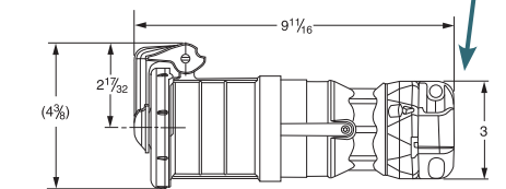
Connector
